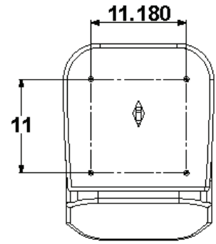
Seat Mounting Bolt Pattern
